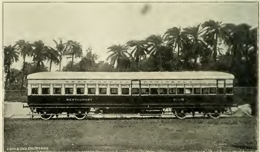
RESTAURANT CAR—GREAT INDIAN PENINSULA RAILWAY.
